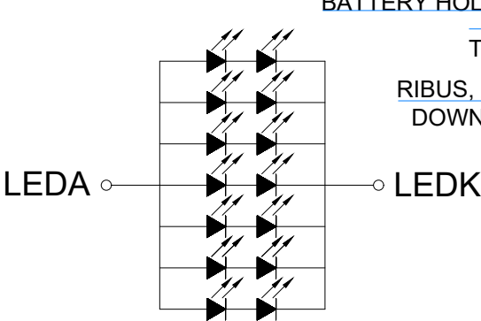
LED Circuit Diagram
